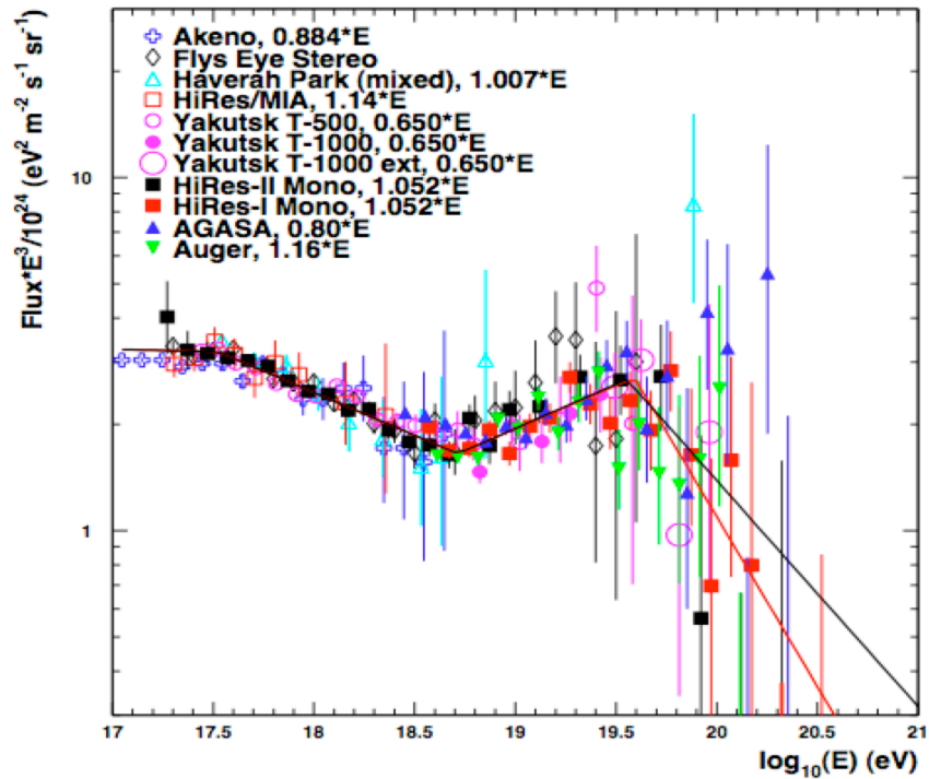
Fig. 1: The spectrum of ultra-high-energy cosmic rays, as measured by several experiments [5]. Every cosmic ray with an energy shown in this plot, namely above 10^{17} eV, liberates in its collision with the atmosphere more energy in its centre-of-mass frame than does a proton-proton collision at the LHC.
