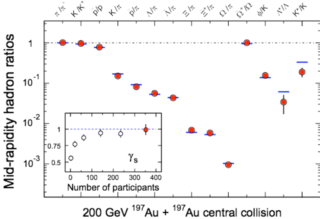
Fig. 2: The relative amounts of different particles and antiparticles produced at RHIC. All the measurements (red points) agree very well with a simple thermal model (blue lines) with an effective temperature around 1.6 trillion degrees, in line with theoretical calculations, and a net nucleon (quark) density that is lower than in previous, lower-energy experiments. The inset shows that the fraction of strange quarks has saturated at the same density as up and down quarks. Figure taken from [3].
