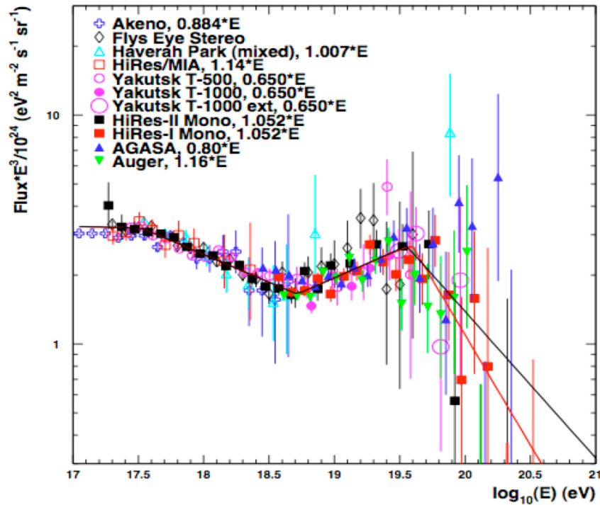
Fig. 1: The spectrum of ultra-high-energy cosmic rays, as measured by several experiments [5]. Every cosmic ray with an energy shown in this plot, namely above 10^{17} eV, liberates in its collision with the atmosphere more energy in its centre-of-mass frame than does a proton-proton collision at the LHC.
